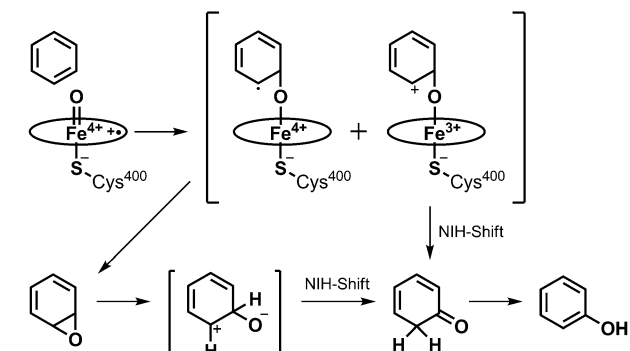
Scheme 1. Proposed reaction mechanism for benzene hydroxylation by P450BM3. [19e]
